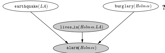
Figure 12: Network reduction with value-insensitive pruning
