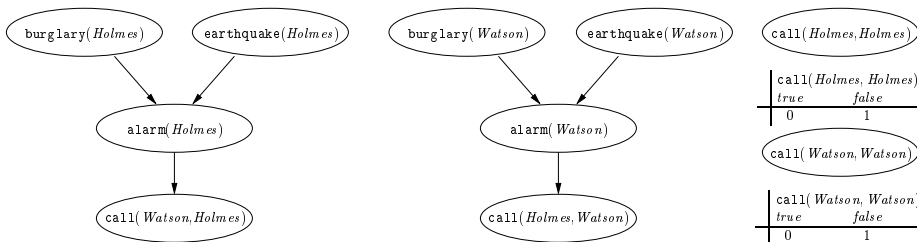
Figure 2: A full instance of a prm for D = \{\text{Holmes}, \text{Watson}\}
