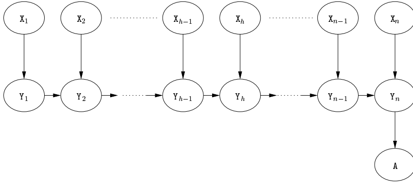
Figure 10: Computation network for mean
