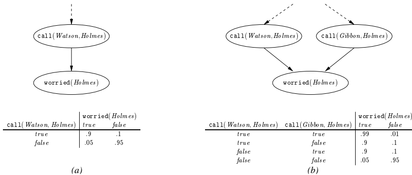
Figure 5: The worried( Holmes ) node in two different domains
