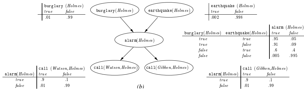
Figure 1: Different instances of the same basic model
