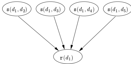
Figure 6: The first network representation of P_{\mathcal{D}}^{\Phi}
