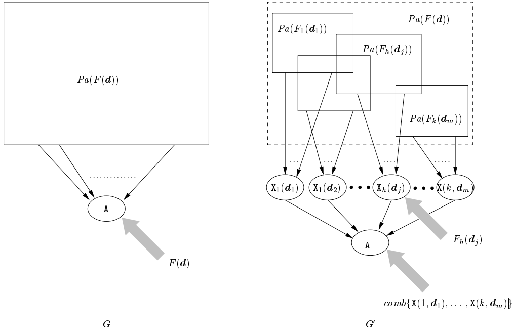
Figure 8: The first decomposition step
