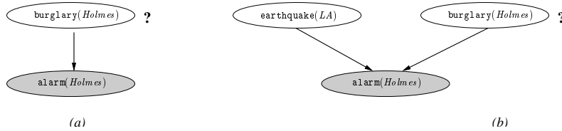
Figure 13: Value-sensitive network reduction
