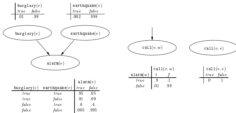
Figure 4: Template representation of introductory prm
