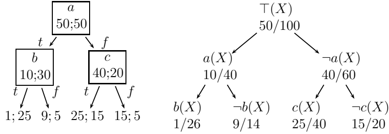
Figure 3: Decision tree and TET discriminant d_+
