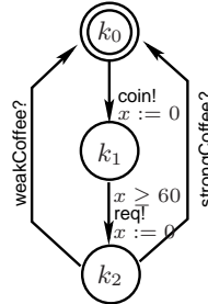
(b) Example environment \mathcal{E}_c
