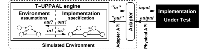
(a) Automated testing of an embedded system.
