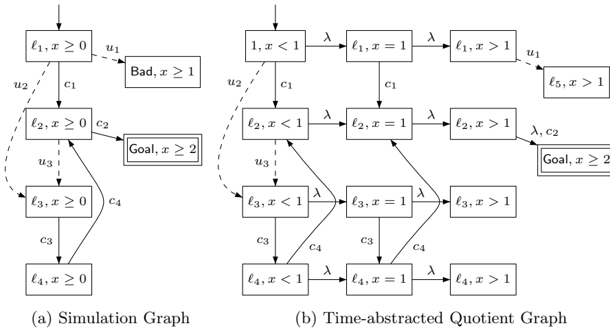
Fig. 2. Simulation and time-abstracted quotient graph of Fig. 1 ( \lambda is for time elapsing)
