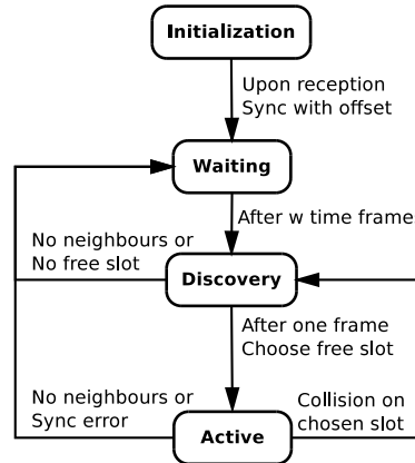
Fig. 11: LMAC protocol phases.
