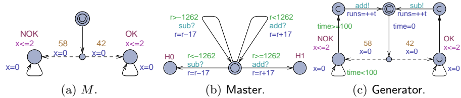
Fig. 3: Sample model M (a) satisfying \Pr[\leq 100](\diamond OK) = 0.42 and modeling SMC of M (b,c) with respect to H_0: \Pr[\leq 100](\diamond OK) \geq 0.5 with 0.05 as level of significance and [0.49, 0.51] as indifference region.
