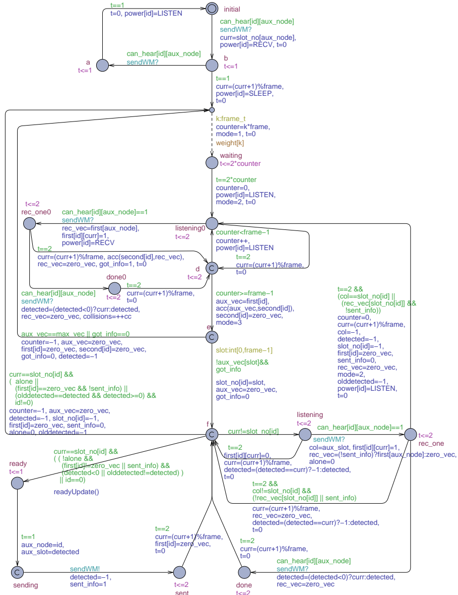
Fig. 14: LMAC node model.
