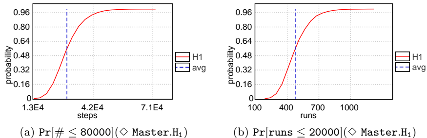
Fig. 4: Cumulative probability plots over number of steps and runs.
