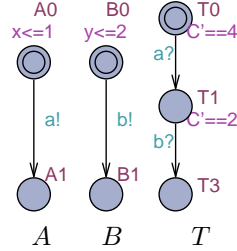
Fig. 1: An NPTA, (A|B|T) .
