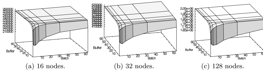
Fig. 15: Estimated processor usage times: E[\leq 16000; 150] (max: usage)
