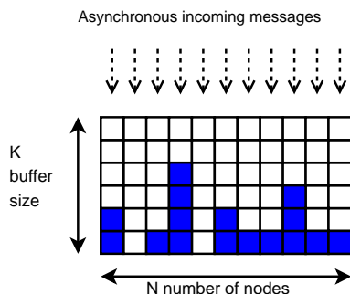
Fig. 6: Buffer of results at the master node.
