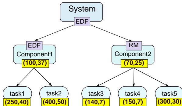
Fig. 1. Example of hierarchical scheduling system.
