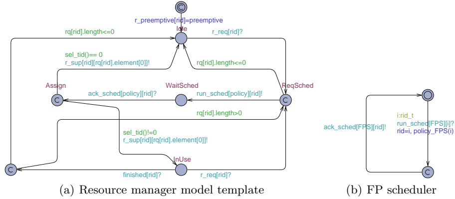
Fig. 7. Resource and scheduling algorithm templates
