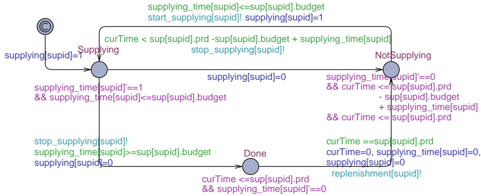
Fig. 3. Non-deterministic supplier template
