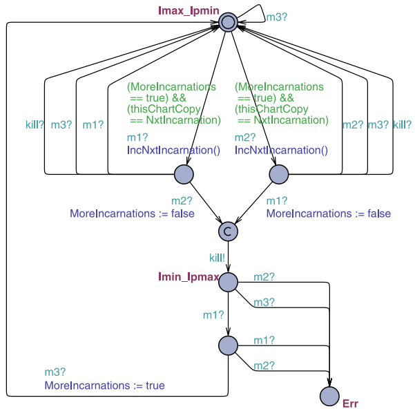
(b) The translated TA template IterativeModeTemplate()
