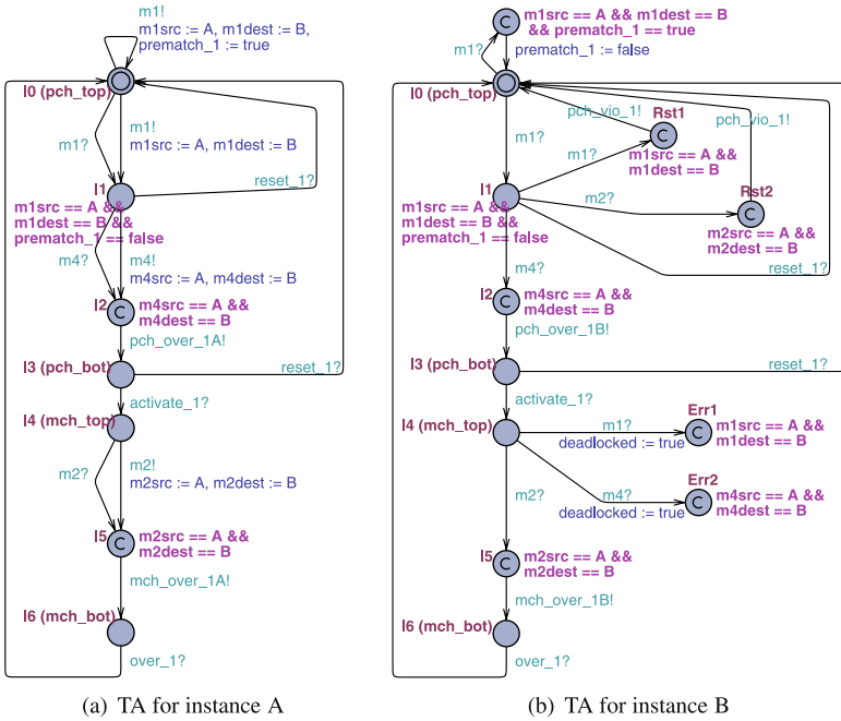
(a) TA for instance A
