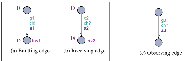
Fig. 12 Coupling emitting/receiving edges in original system model S and the observing edge in observer timed automaton O_L
