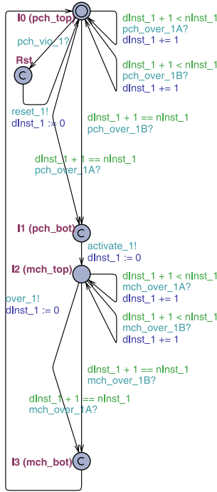
(c) The coordinator automaton
