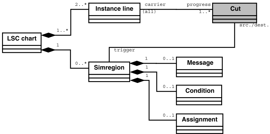
Fig. 6 Class diagram for time-enriched LSC language
