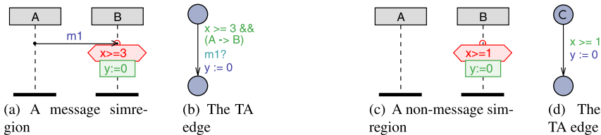
Fig. 8 Translating LSC simregion to TA edge (here “ A \rightarrow B ” denotes that instances A and B are the message sender and receiver, respectively)
