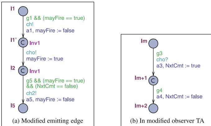
Fig. 15 Further modifications for Fig. 14
