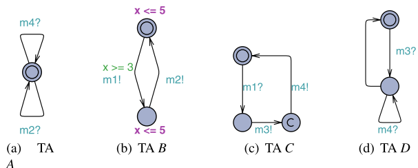
Fig. 2 A real-time system model (network of TAs)
