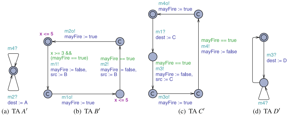
Fig. 16 The modified model S' of the original real-time system in Fig. 2(a)–(d)
