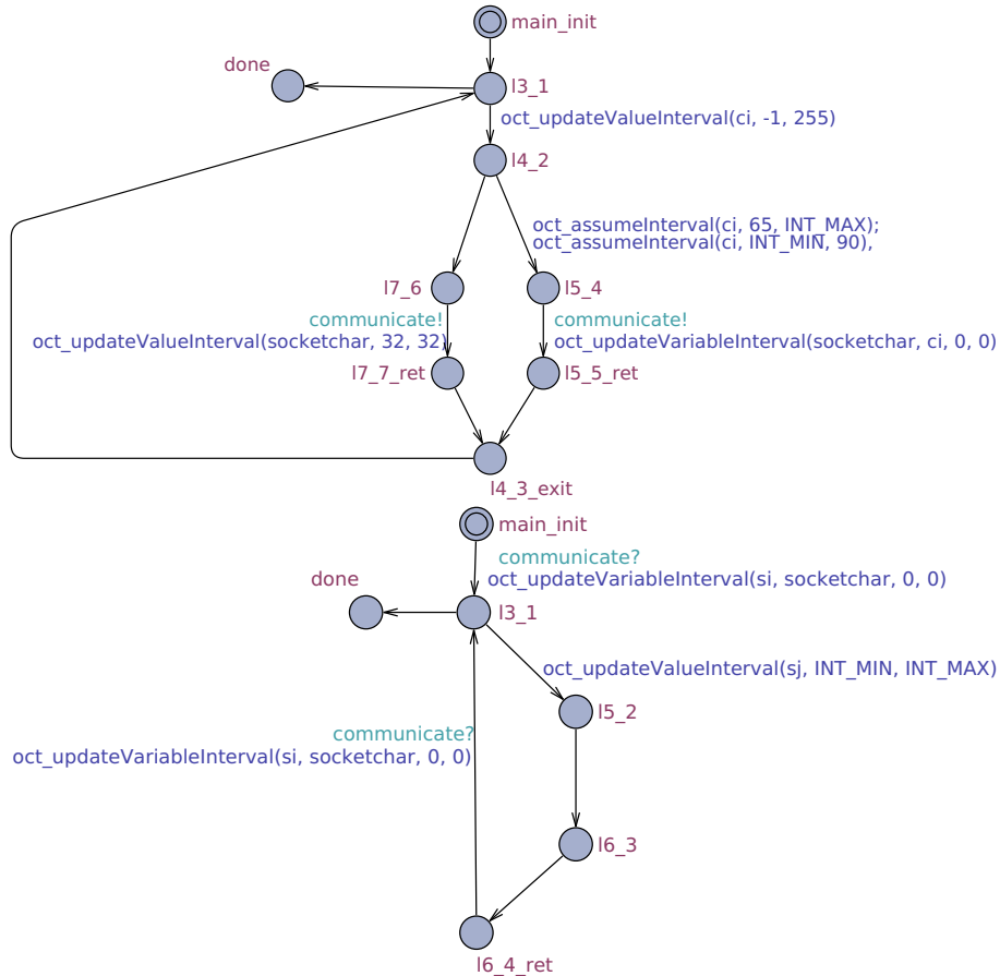
Figure 7.11: The manually composed client and server model of Figure 7.10. The two automata communicate over the octagon variable socketchar and synchronise over the channel communicate .
