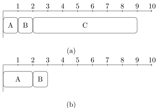
Figure 8.3: Example program run on M_3 . The program is A : MUL R_0, R_0, R_1 ; B : BRZ R_0, C , where C is a linear, data-independent, subprogram summarised into one instruction. The instruction BRZ is interpreted as “branch to C if R_0 is zero”. The two traces are (a) where R_0 = 0 , and (b) where R_0 = 1 .
