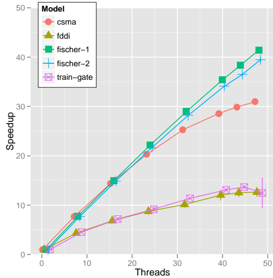
Figure 6.7: Speedups in LTSMIN/opaal
