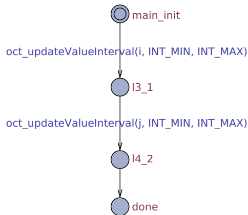
(b) The lattice automaton generated by C2OPAAL when run on the program.
